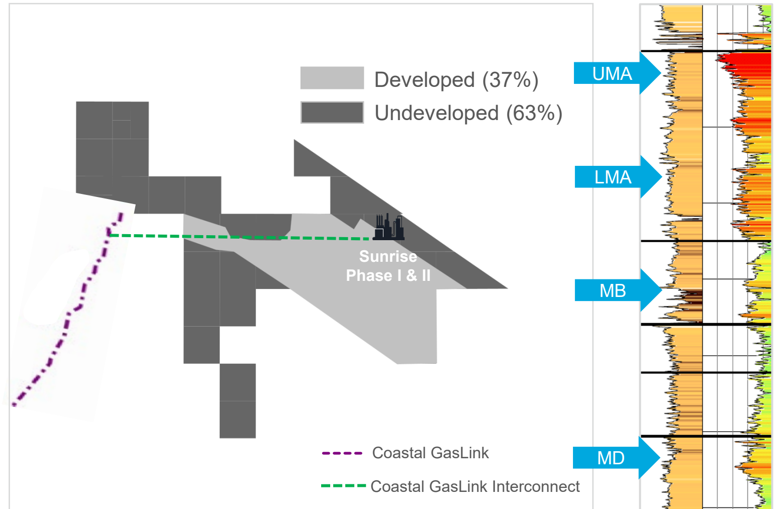
Sunrise Type Well
