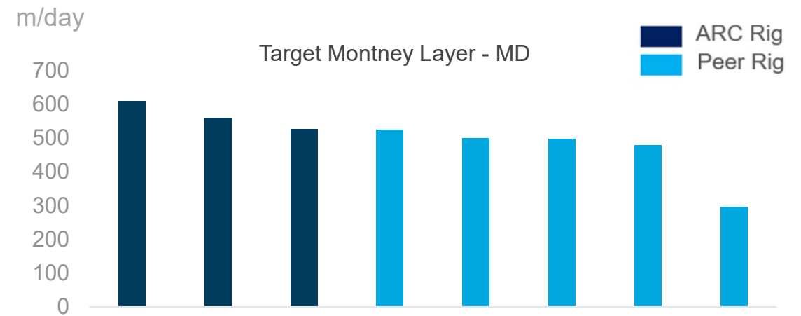
Drilling Efficiency 1 2
